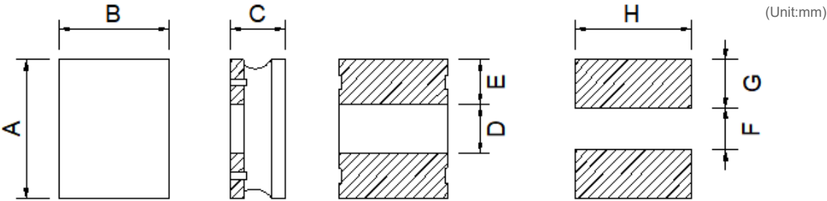
Recommended Land Pattern 推荐焊盘
